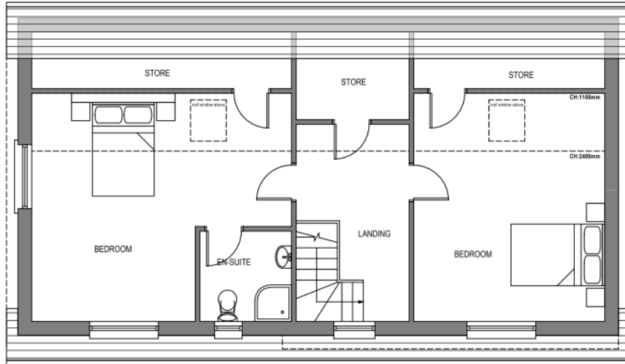
PROPOSED FIRST FLOOR PLAN Scale 1:50
